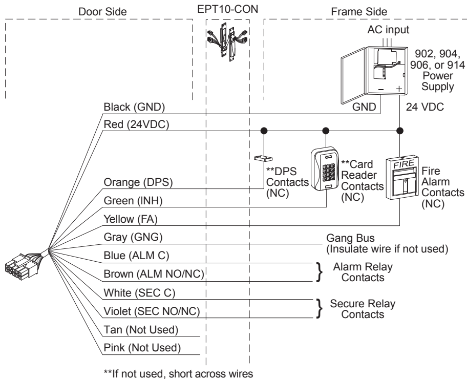
Figure 2. Point-To-Point Diagram, Single Door
